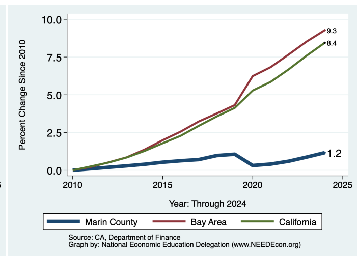
Figure 6 - 2: Housing Growth
