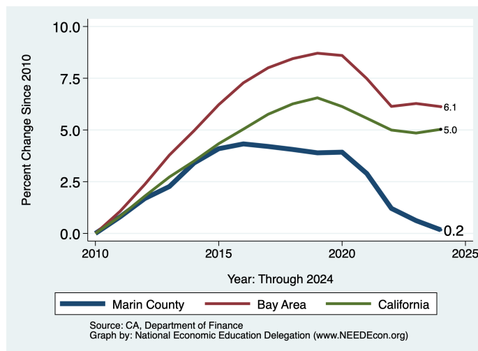
Figure 6 - 1: Population Growth
