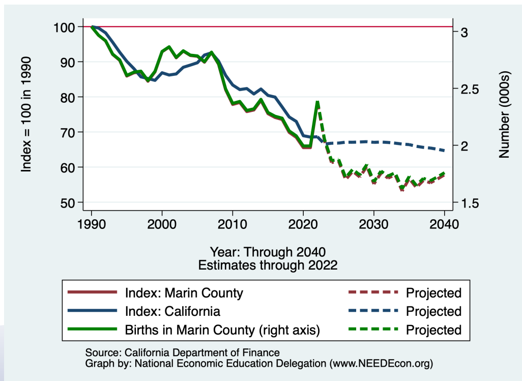
Figure 4 - 7: Birth Projections
